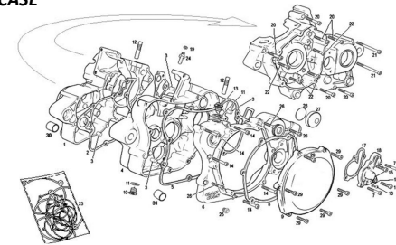
CARTER CRANKCASE
