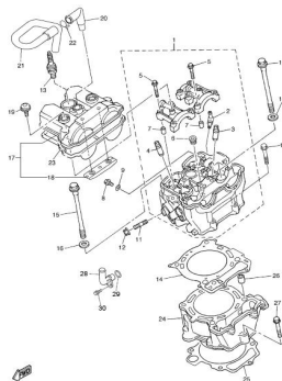
CILINDRO CYLINDER
