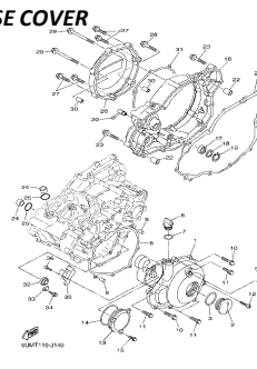
TAPA CÁRTER CRANKCASE COVER
