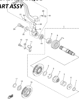
CTO. PEDAL ARRANQUE KICKSTART ASSY
