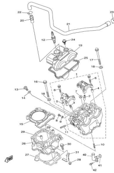
CILINDRO CYLINDER
