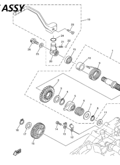
CTO. PEDAL ARRANQUE KICKSTART ASSY
