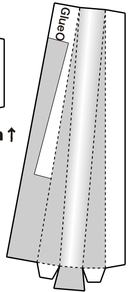
④ Muffler ↓
